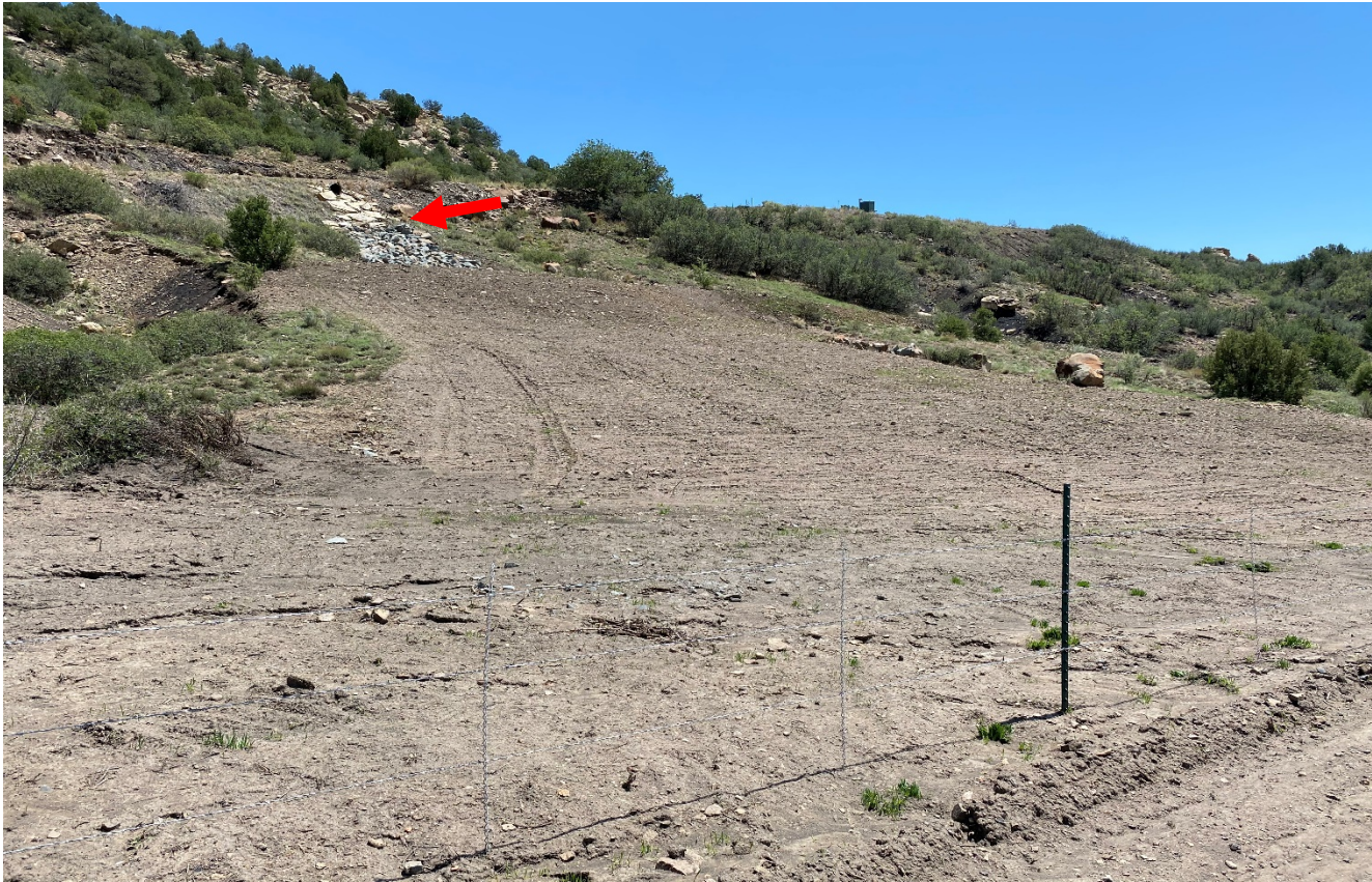
Photo 1. Facing southeast along CR 41.7. This area has been regraded and outlet protection has been installed at the culvert shown at red arrow.
