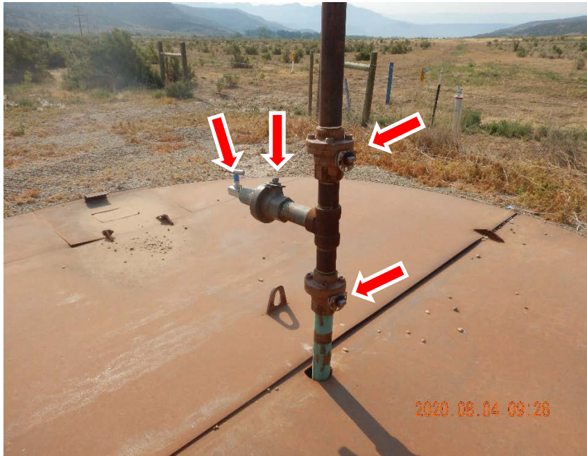
Photo #1 – Valves attached to flowline riser neither locked nor tagged out.
