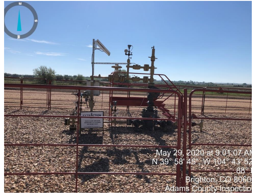
Photo#10 Wellhead
