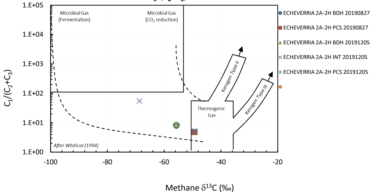
Methane \delta^{13}\text{C} vs \text{C}_1/(\text{C}_2+\text{C}_3) Genetic Classification Plot
