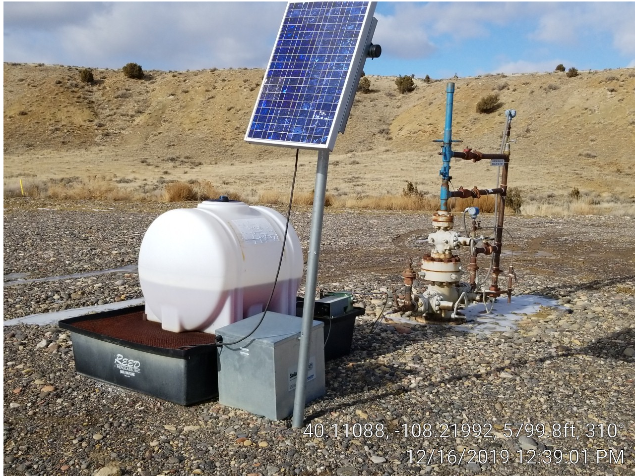
Photo 2. Well head.
