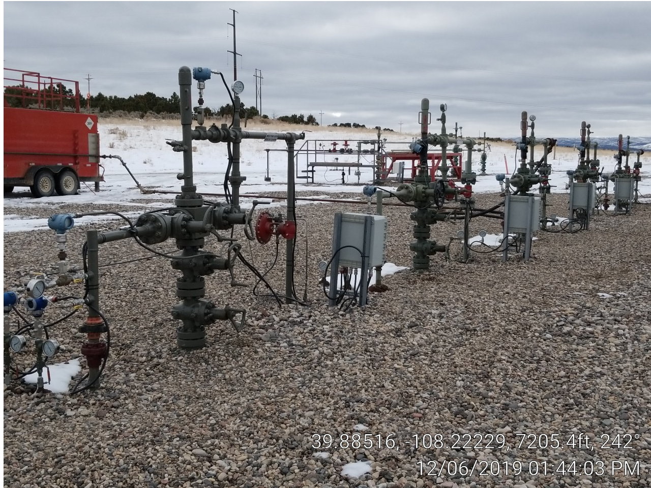
Photo 2. Well heads.
