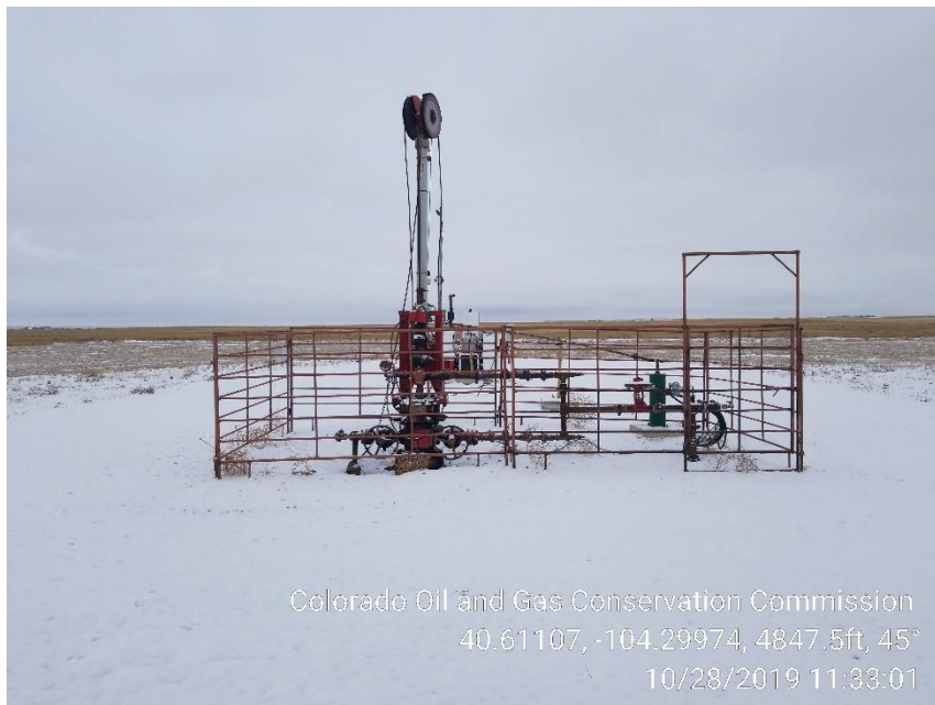
Photo 1 – Pumping Unit
