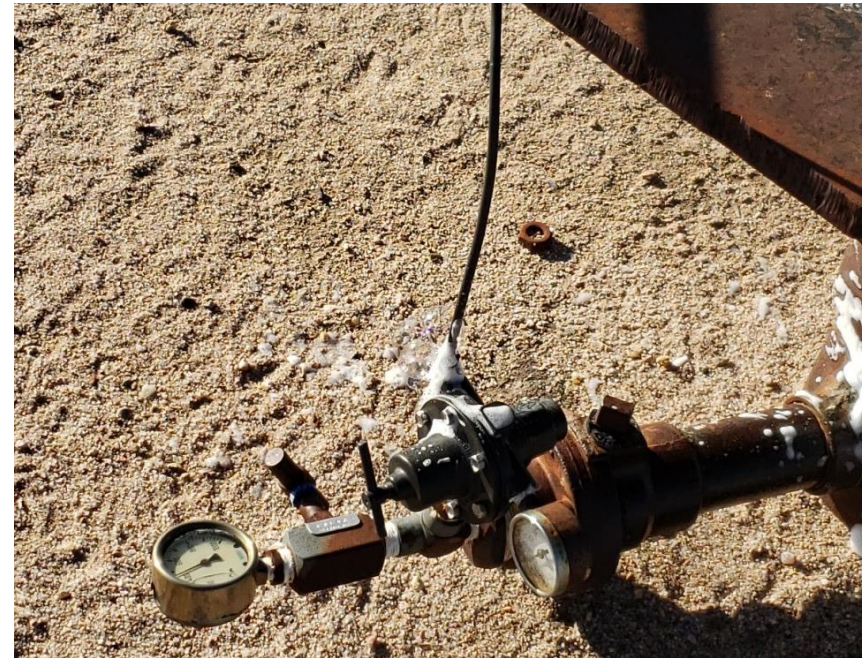
Photo #3 Active leak at the Meco regulator stainless fitting.
