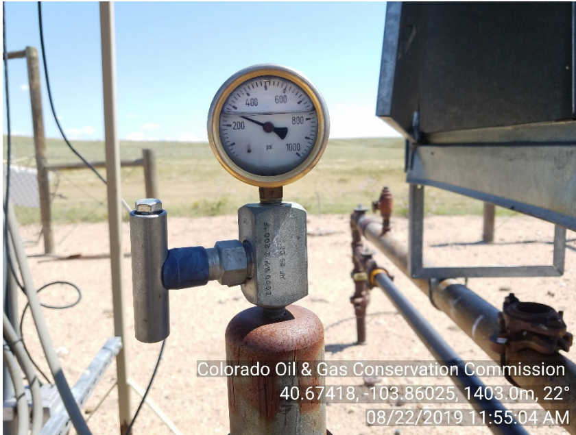
Photo #3 Lilli Unit 9-9 UIC - Injection Wellsite Shut-In | SI Tbg. Press: 260#
