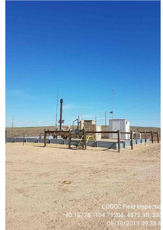
Photo 3 Production Equipment
