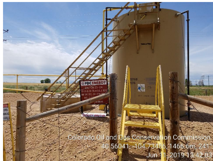
Photo 2: Tank Battery
