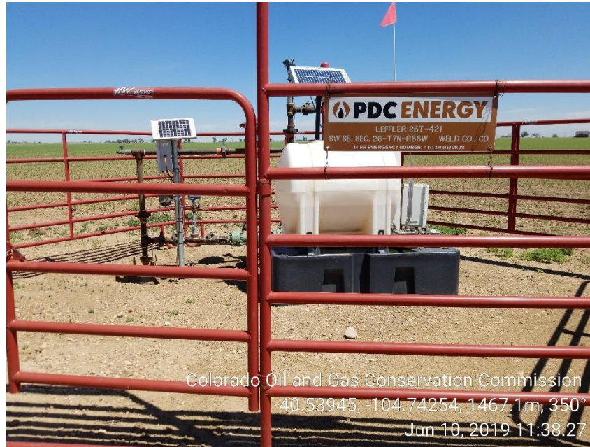
Photo 1: Wellhead with methanol pump
