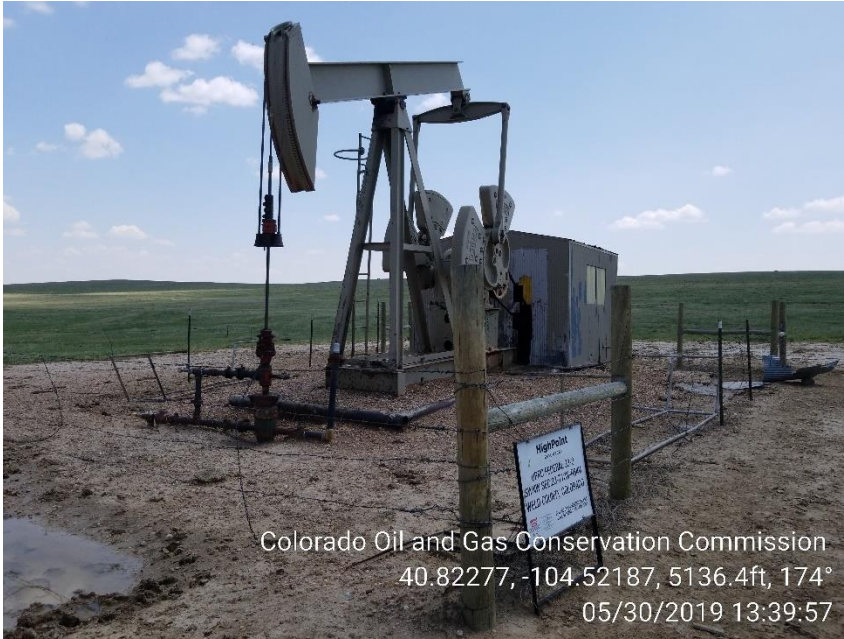
Photo 1 – Pumping Unit
