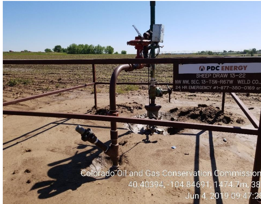
Photo 1: Wellhead
