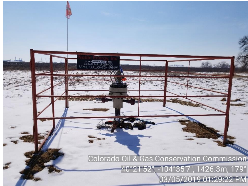
Photo 1: Wellhead
