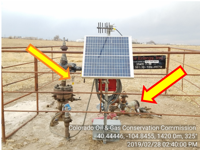
Photo #3 State 7-36 (05-123-11980) Wellsite Temporarily Abandoned | TA Unused Equipment Orange Decommission tag NOT present
