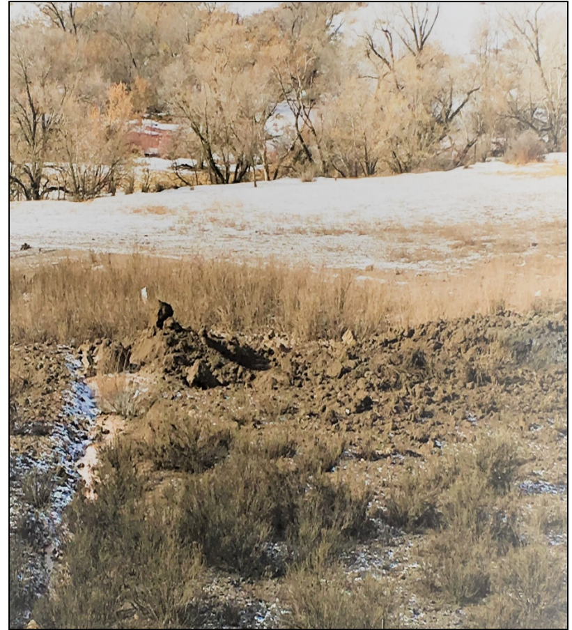
Closer view of Pipeline ruptured area
