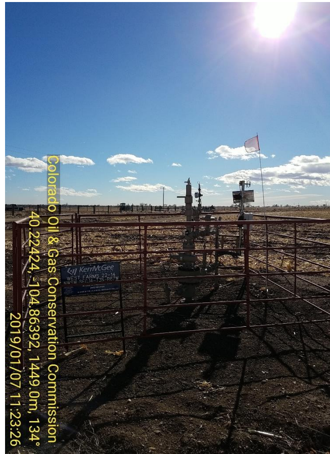
Photo 1 Wellhead
