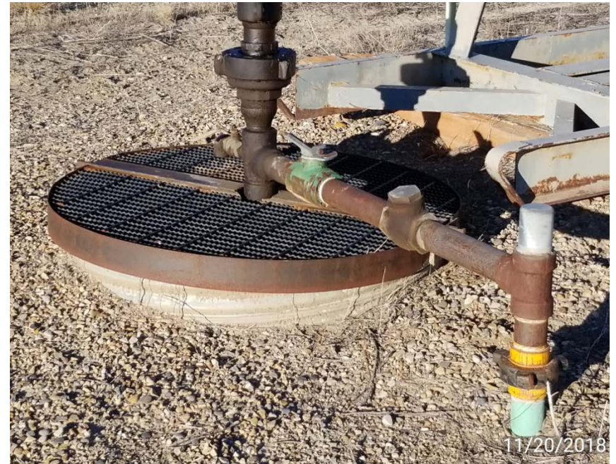
Photo 2. Wellhead not venting. No valve below cellar. Valve above cellar closed.
