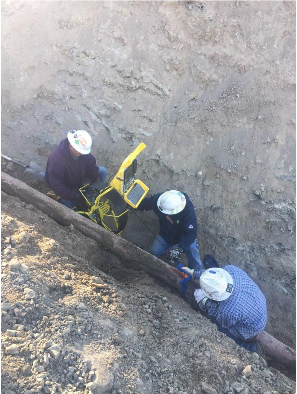
Inspection work on 6" PW transfer line being completed by BP personnel.
