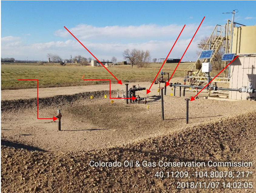
PHOTO 3: There are 6 unmarked unused risers between meter house and heated separator
