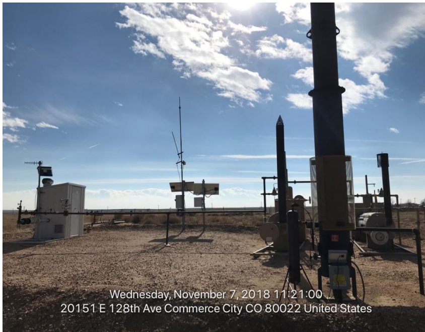
Photo#3 Separator/ECD/Automation RTUs/Gas Meter
