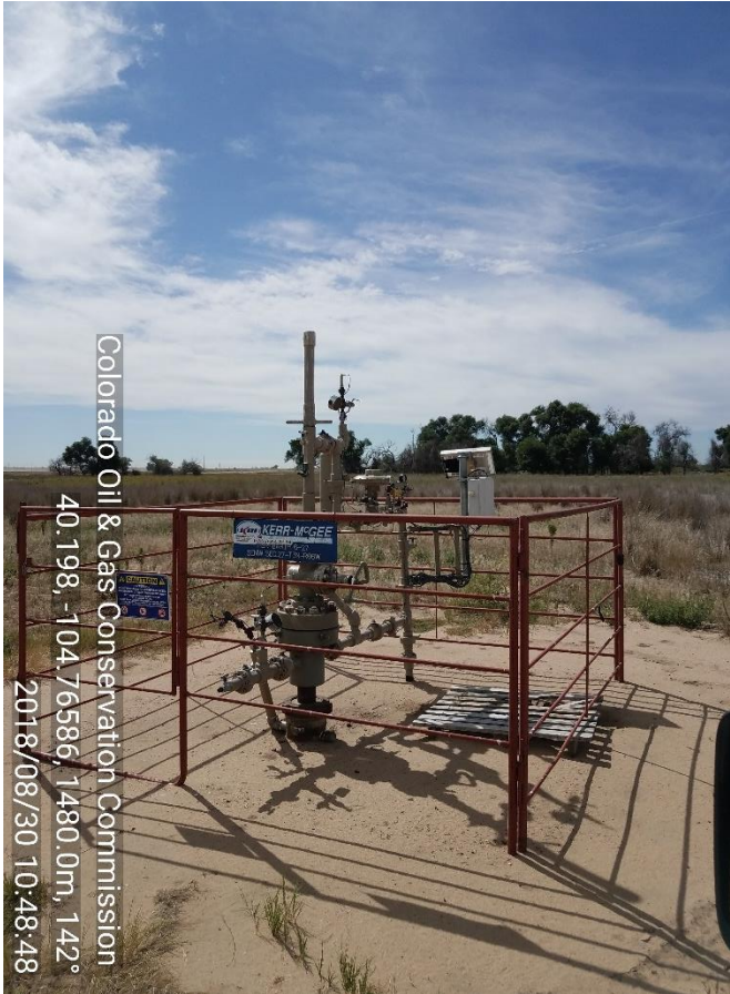
Photo 1 Wellhead
