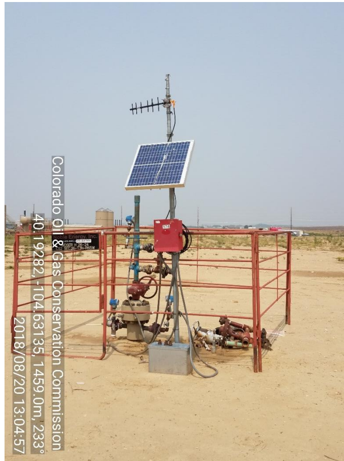
Photo 1 Wellhead
