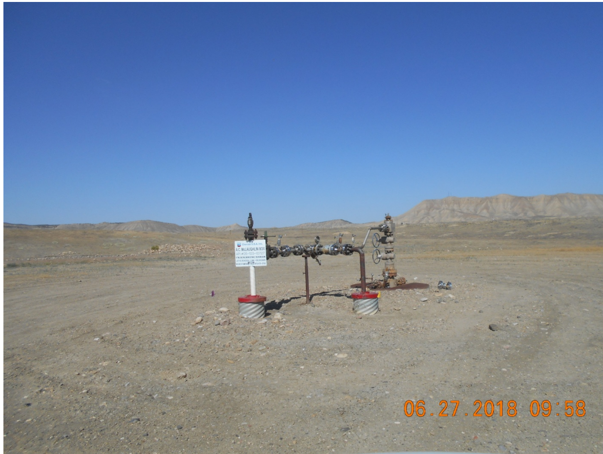
Injection Wellhead
