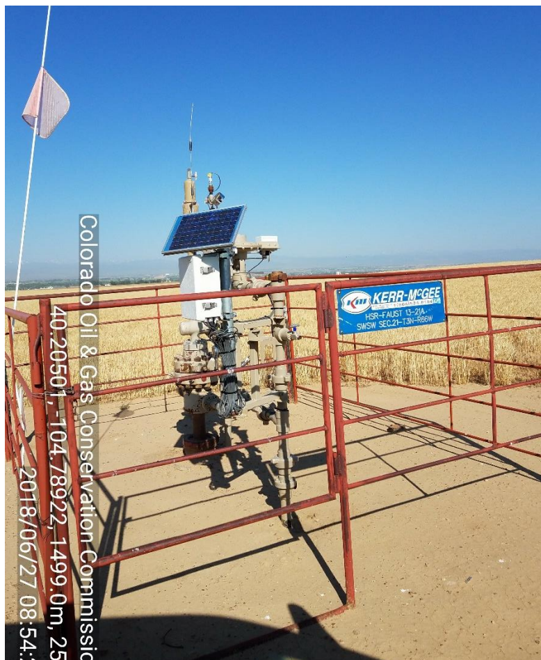
Photo 1 Wellhead
