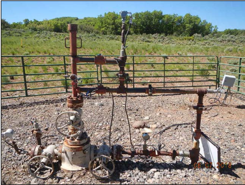
Photo 1. Wellhead.
