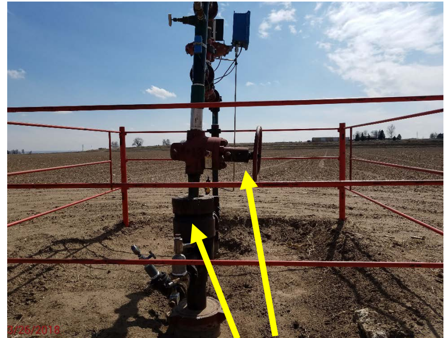
Kammerzell 29-4 H6 wellhead facing S. Casing head has audible leak with stain. Master valve stem appears to be dripping fluid
