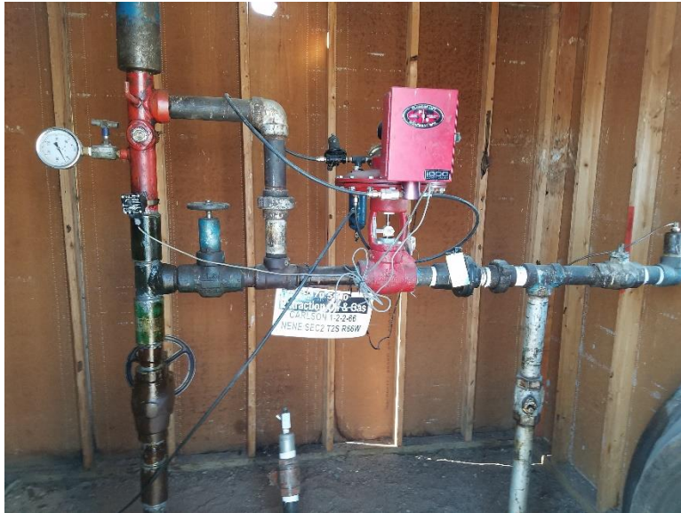
Photo 1. Wellhead looking south
