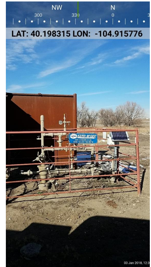
Photo 3 Wellhead API 05-123-19183
