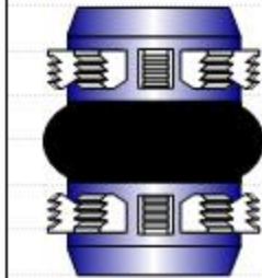
7-5; KLINE 5 1/2" RETRIEVABLE BRIDGE PLUG
