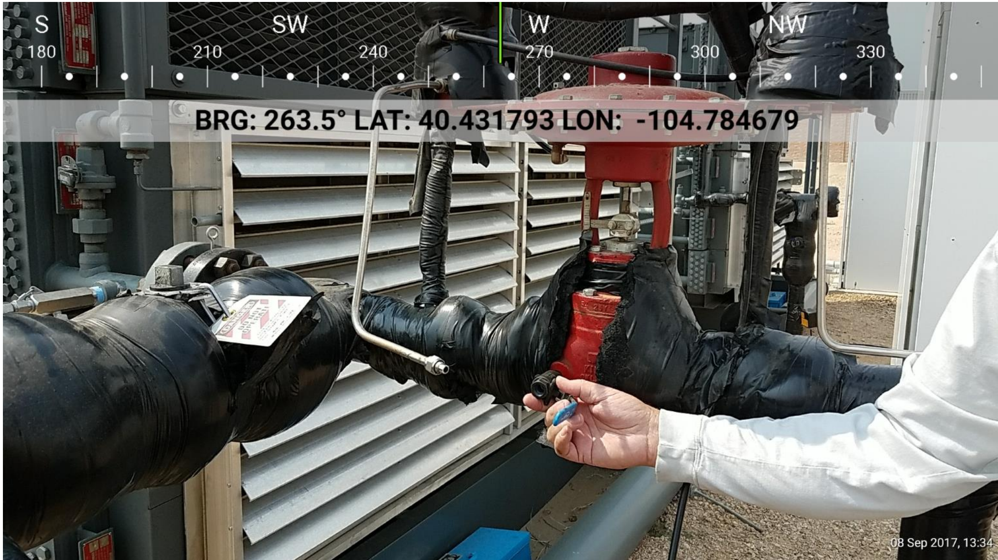
Close view of area where nipple failed.
