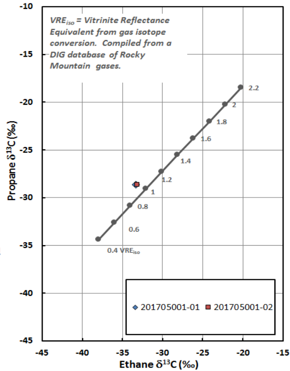
Ethane - Propane Maturity Plot
