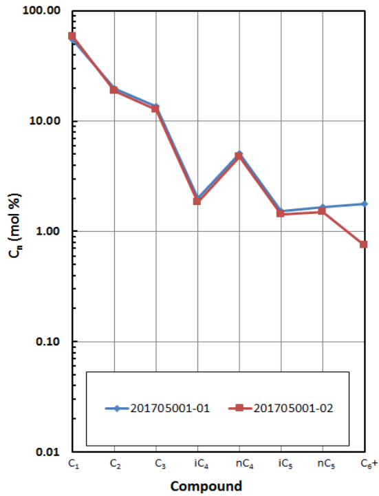
Hydrocarbon Composition Plot
