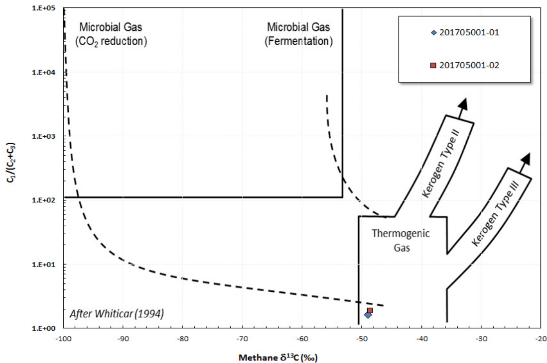
Methane d13c vs C1/ (C2+C3) Genetic Classification Plot
