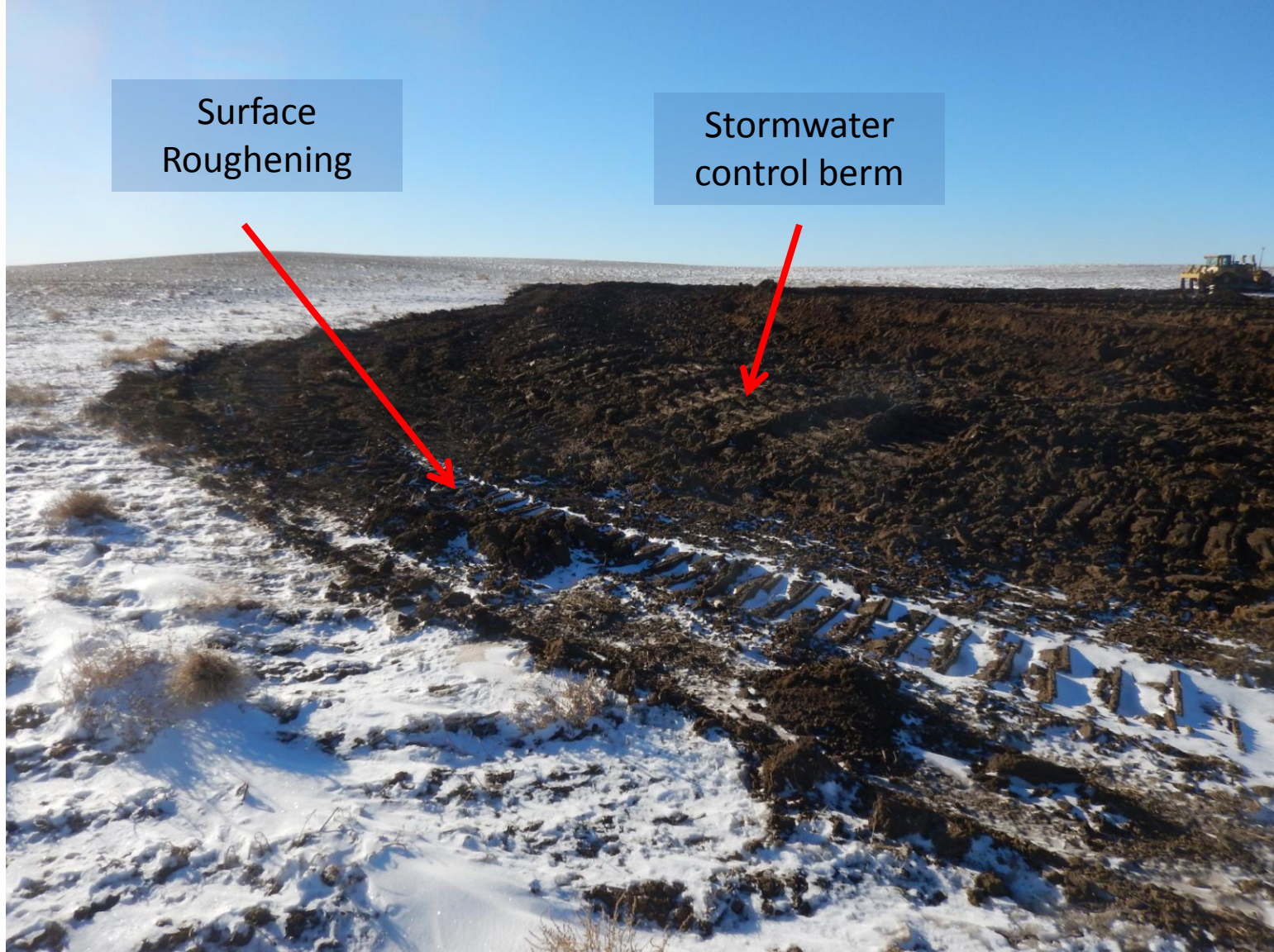
Figure 15: Photo taken from northeast corner of location, facing south. Photo of stormwater BMPs. Note inadequate surface roughening, downslope of stormwater control berm.
