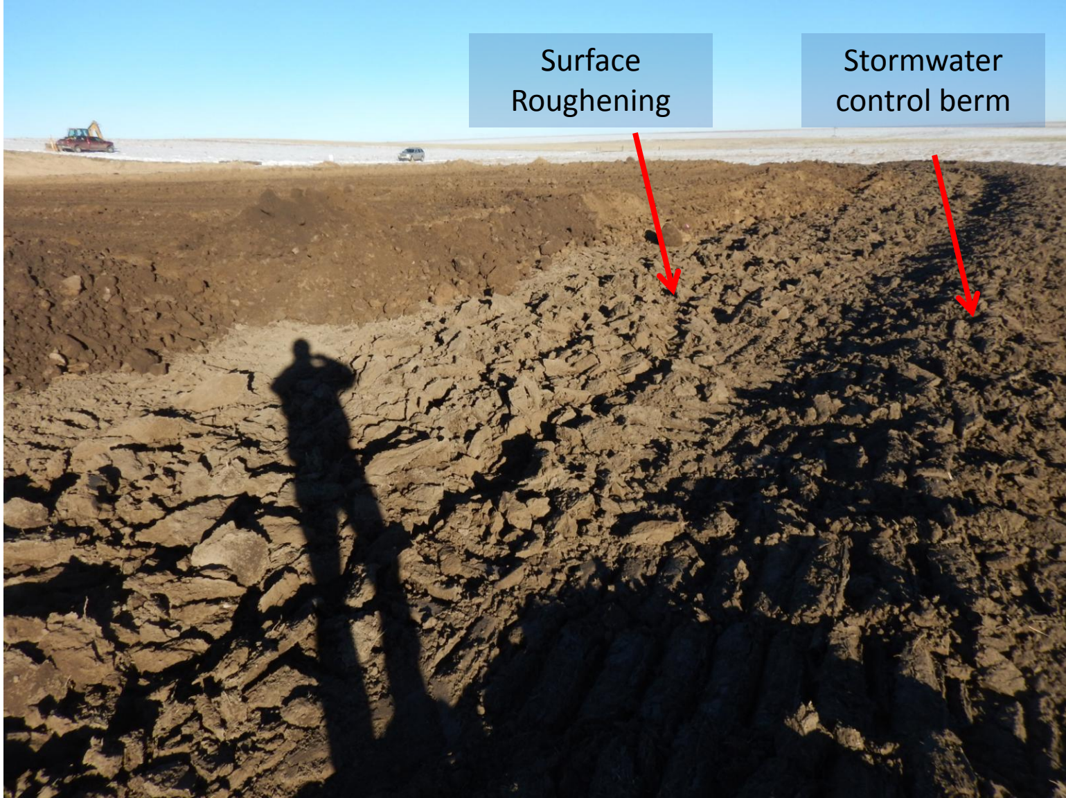
Figure 14: Photo taken from stormwater control berm on east end of location, facing north. Photo of adequate surface roughening BMP up slope of stormwater control berm..
