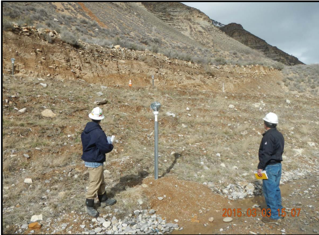
Wind-powered SVE
