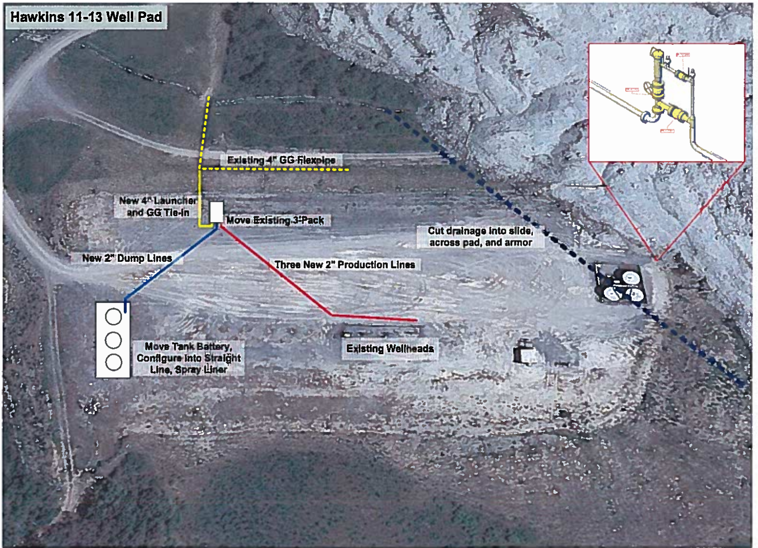
Figure 2 – Facilities Layout
