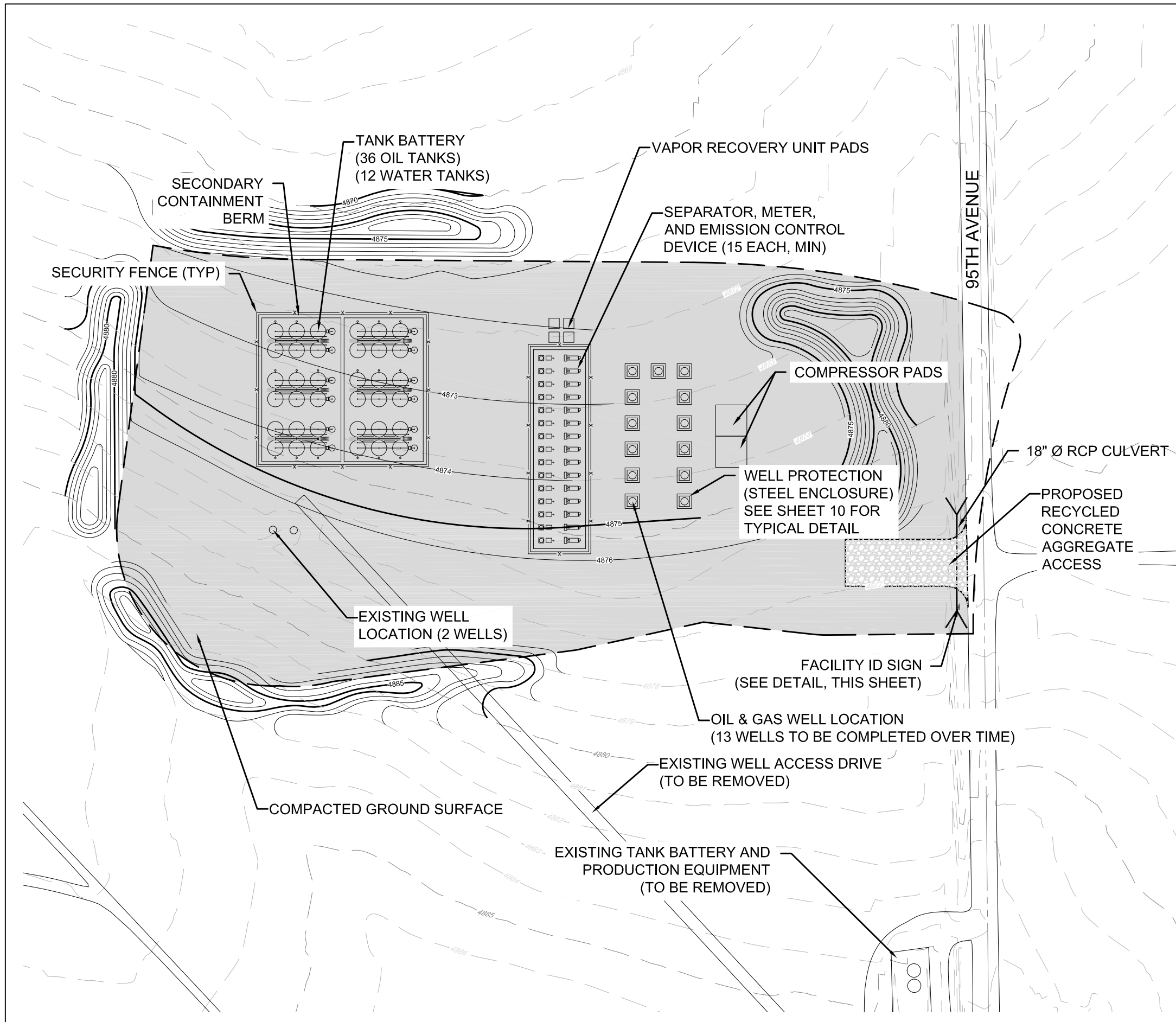
SEPARATORS, METERS, AND EMISSION CONTROL DEVICE CONTAINMENT BERM (TYP)
