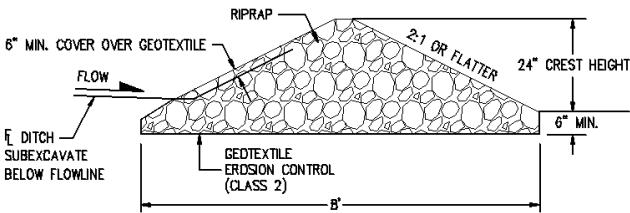
SECTION DETAIL
