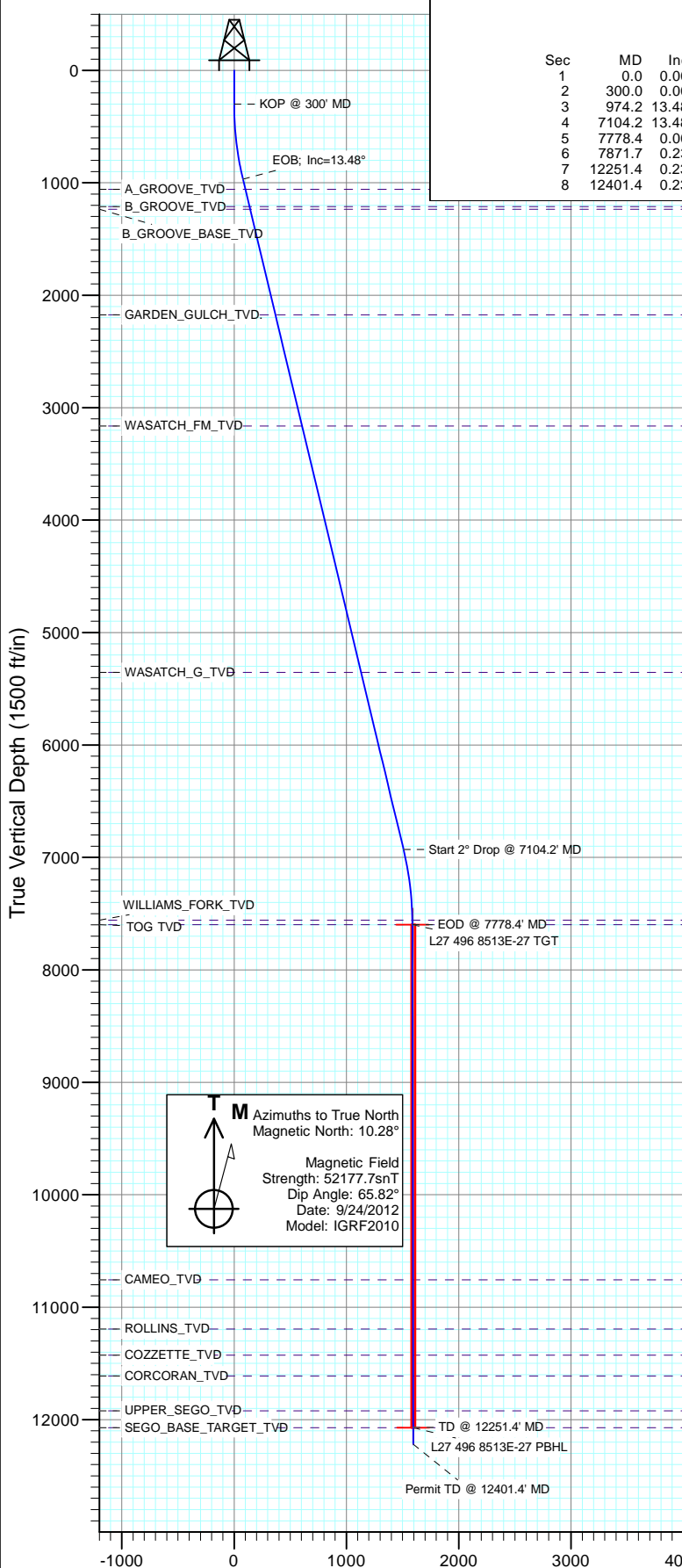
Vertical Section at 170.43° (1500 ft/in)
