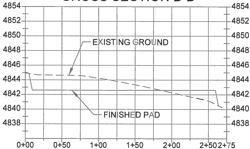
CROSS SECTION B-B
