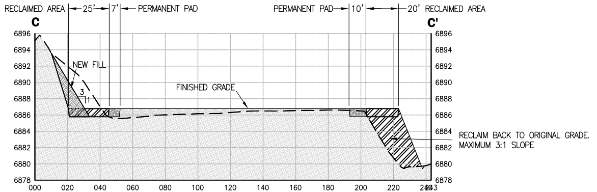
SECTION C-C' RECLAMATION
