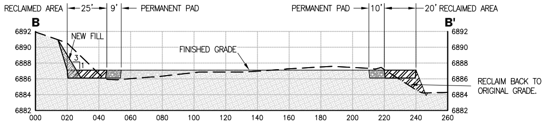
SECTION B-B' RECLAMATION
