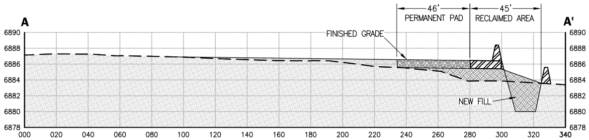
SECTION A-A' RECLAMATION
