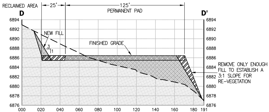
SECTION D-D' RECLAMATION
