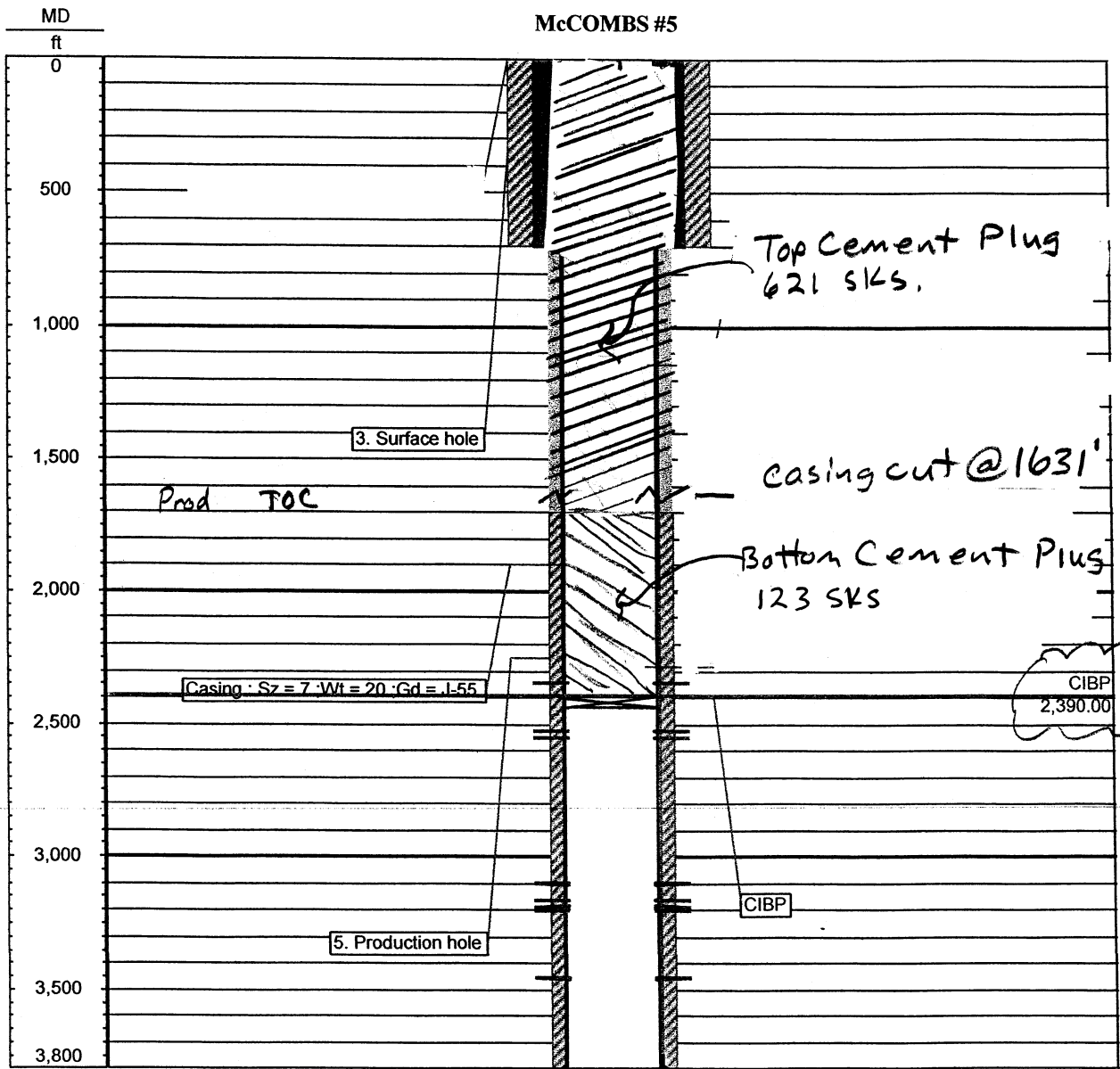
Wellbore with intended plugs
