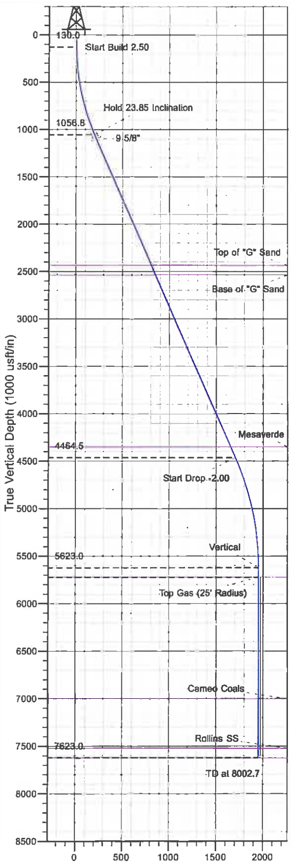
Vertical Section at 99.39° (1000 usft/in)
